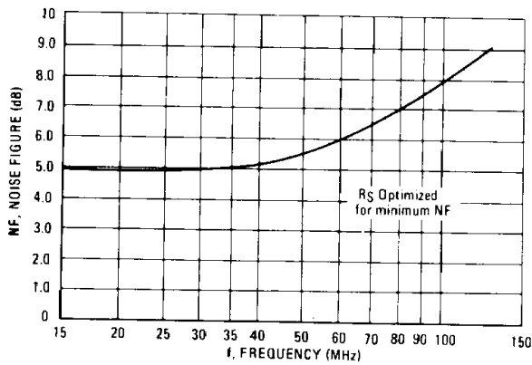
FIGURE 11 – NOISE FIGURE versus FREQUENCY
