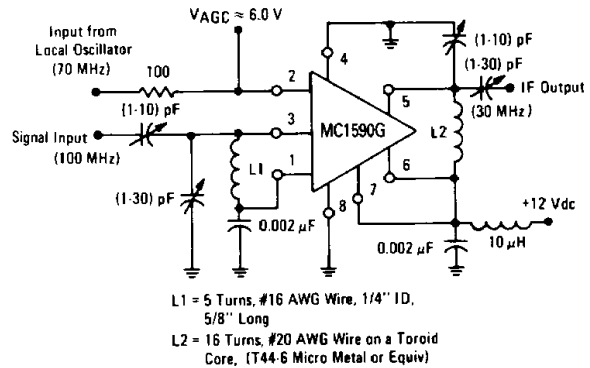
FIGURE 28 — 100 MHz MIXER
